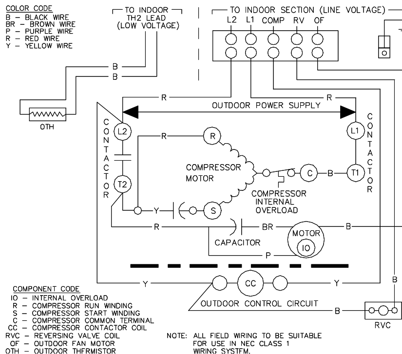
Circuit (Typical Wring For Use With Ductled Indoor Section - *Note: 24 Volt Contactor is Field Supplied.
