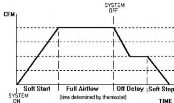
Air flow delivered to the system by the AEPT air handler for a typical cooling/heating cycle.
