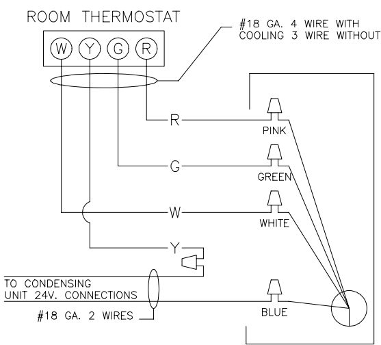
Thermostat Anticipator Setting for optional heat kits 15 KW and above
