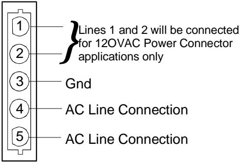
5 PIN CONNECTOR
