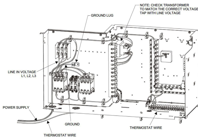
HP/AC Control Box
