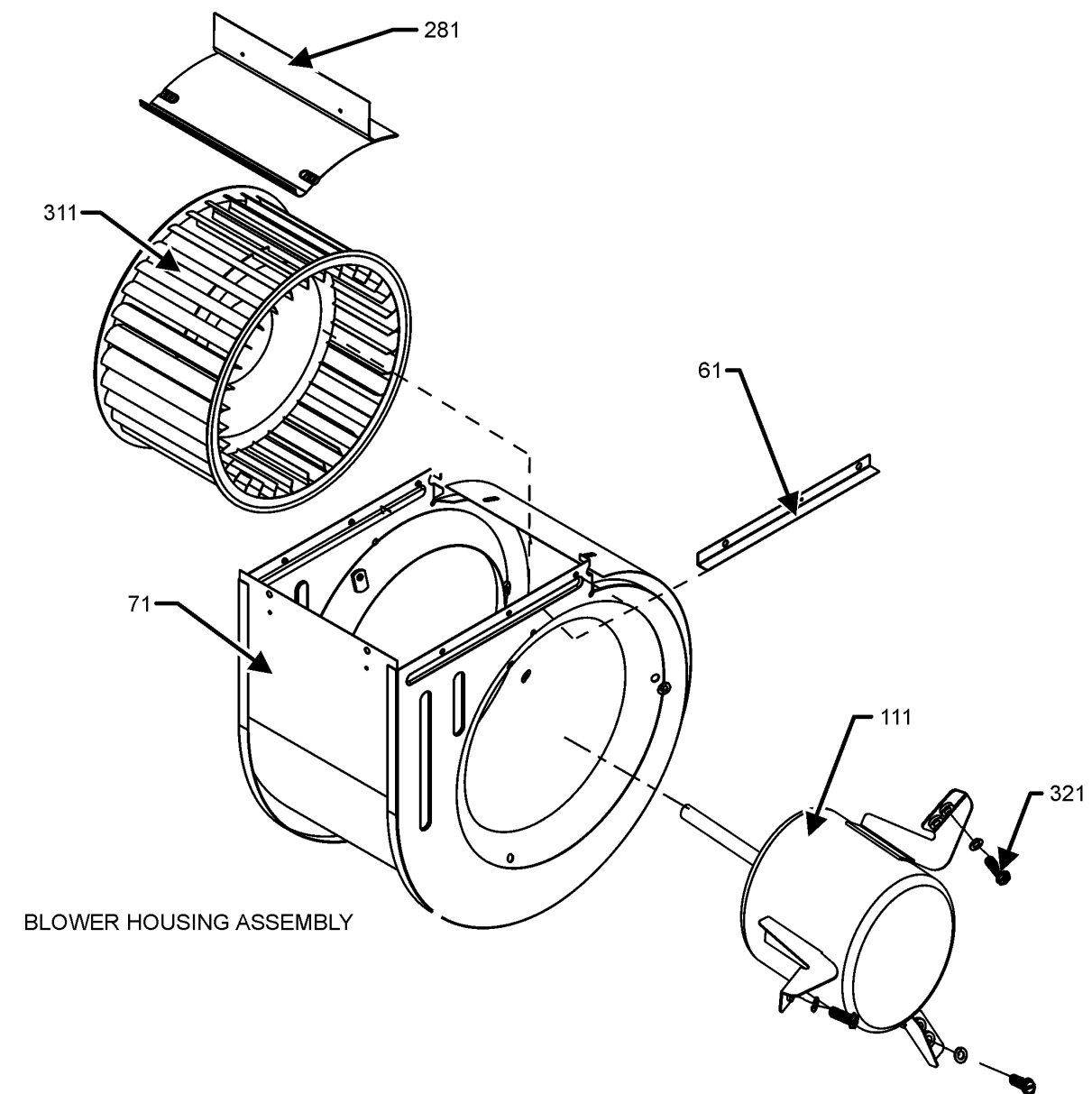
BLOWER ASSEMBLY
