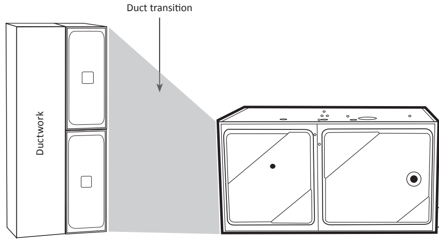
Duct transition for side flow dual filter installation furnace/air handler application
