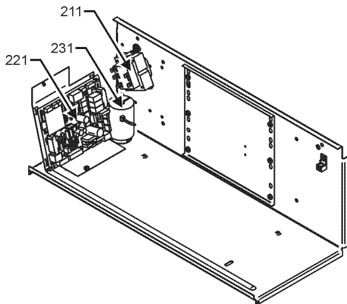
CONTROL PANEL ASSEMBLY
