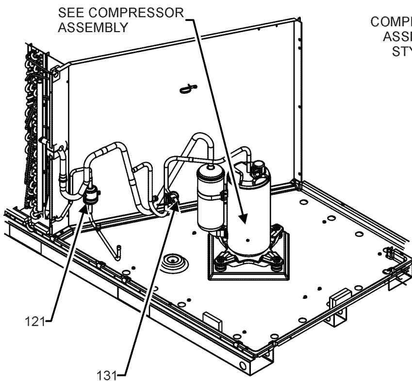
TUBING ASSEMBLY
