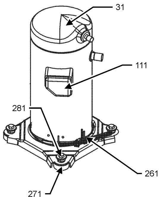
COMPRESSOR DETAIL
