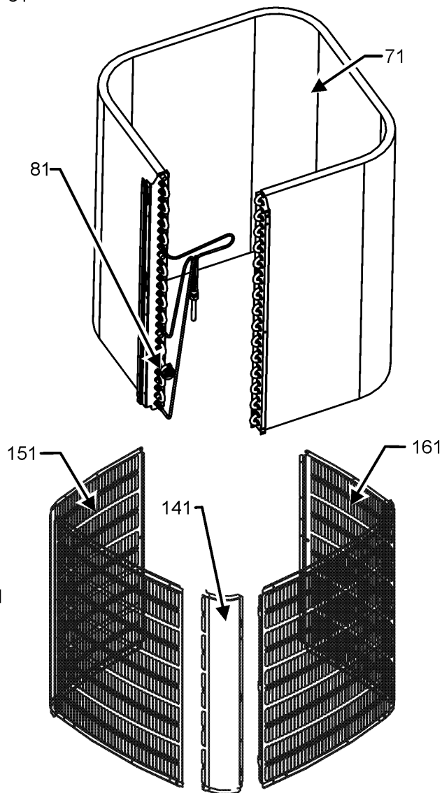
LOUVER PANEL ASSEMBLY STYLE 2
