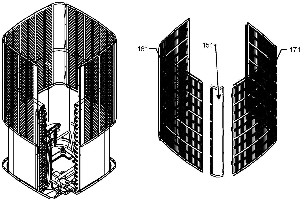
LOUVER PANEL ASSEMBLY STYLE 1
