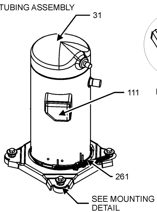
COMPRESSOR DETAIL
