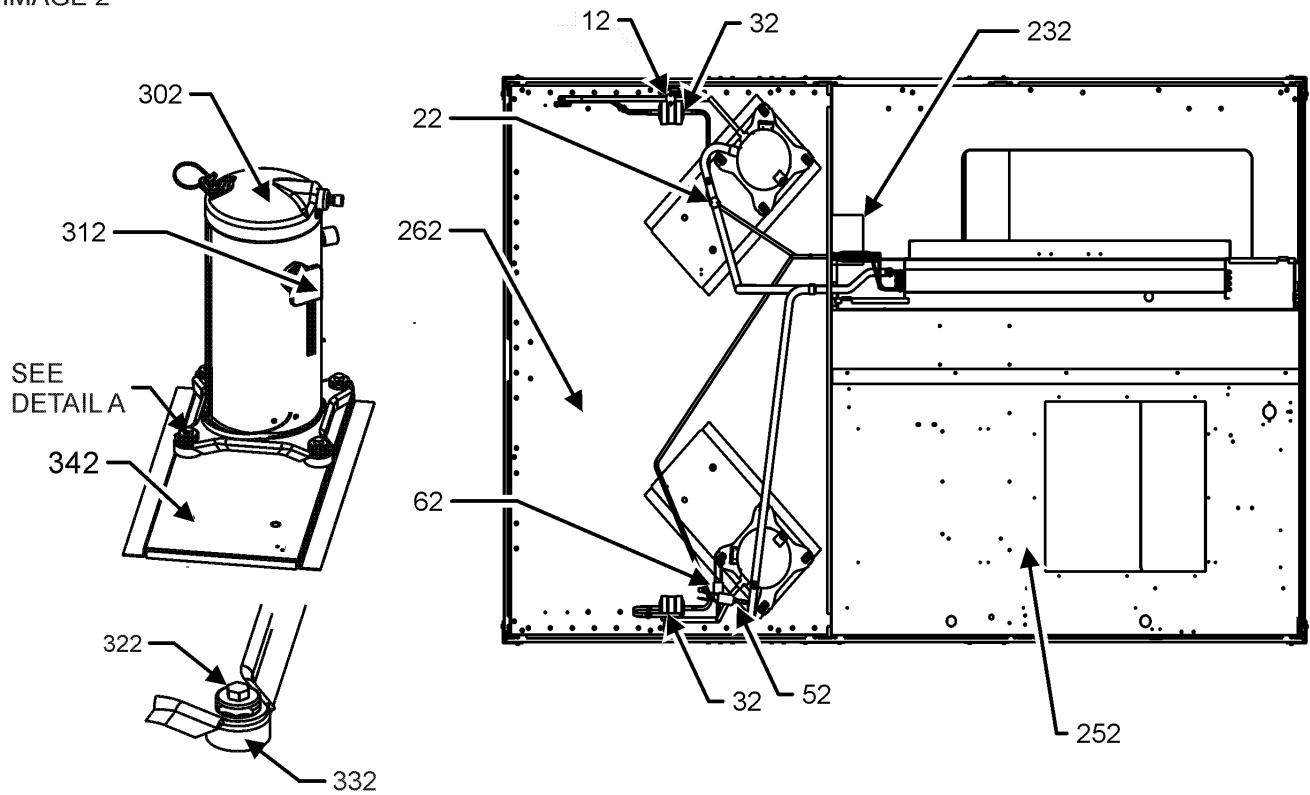
DETAIL A
