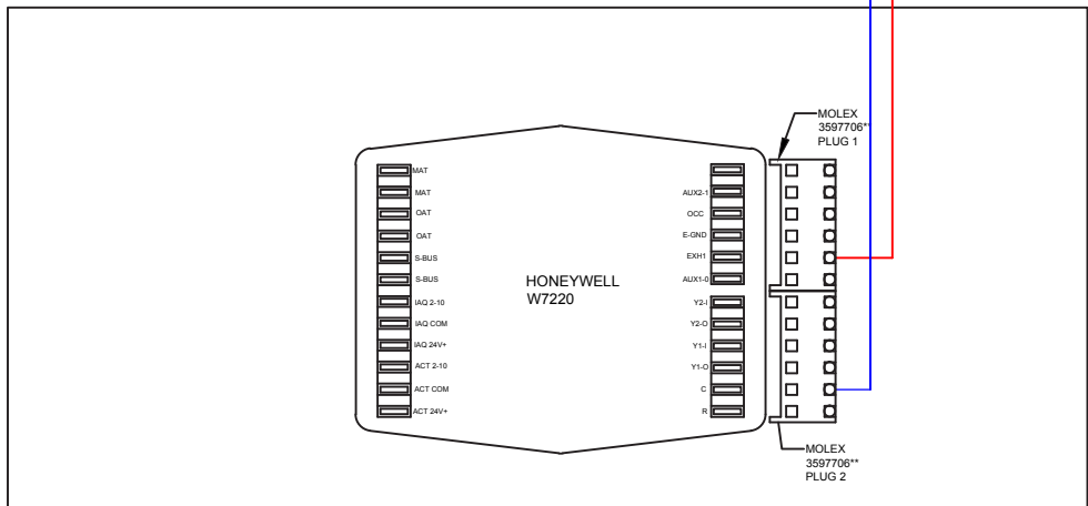
SPE1803004 Wiring Diagram
