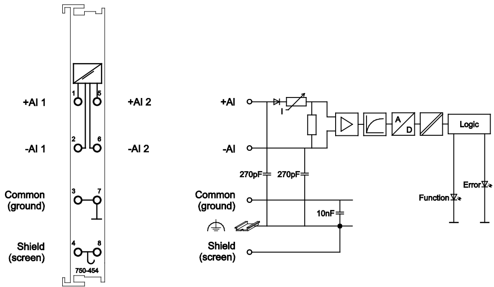
Figure 5: Schematic diagram
