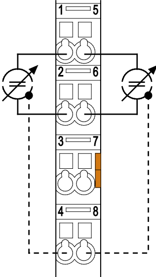
Figure 10: Connection example 750-454
