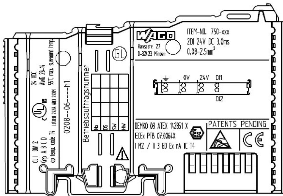
Fig. 2.2.2-3: Example for lateral labeling of bus modules (750-400, 2 channel digital input module 24 V DC)
