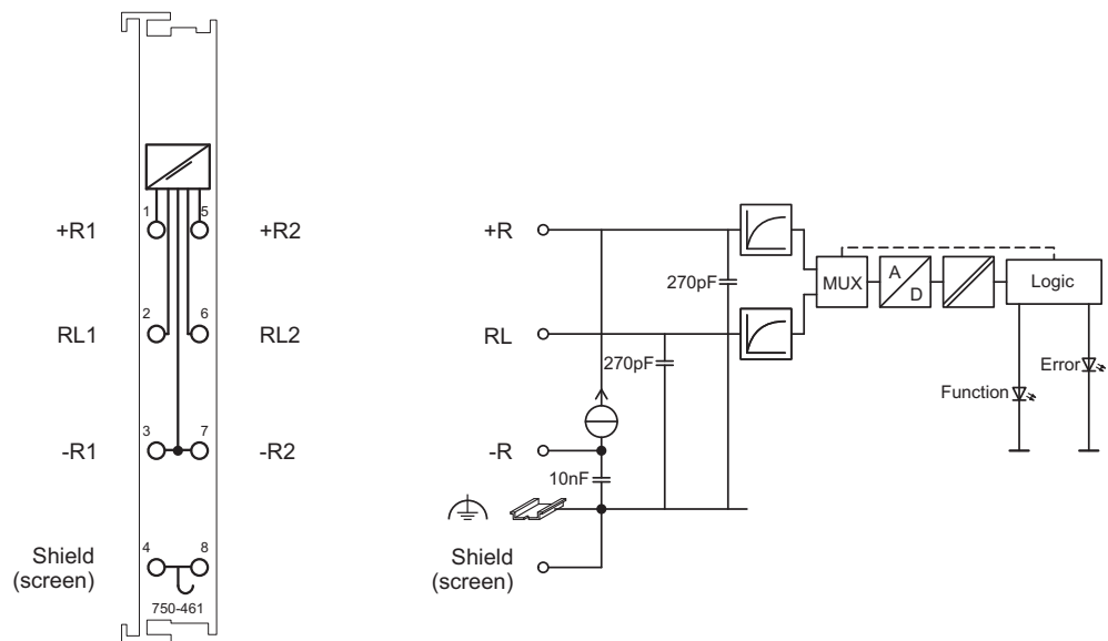
Fig. 2.1.2-3: Schematic Diagram
